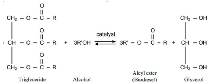
Figure 2: Transesterification Reaction
